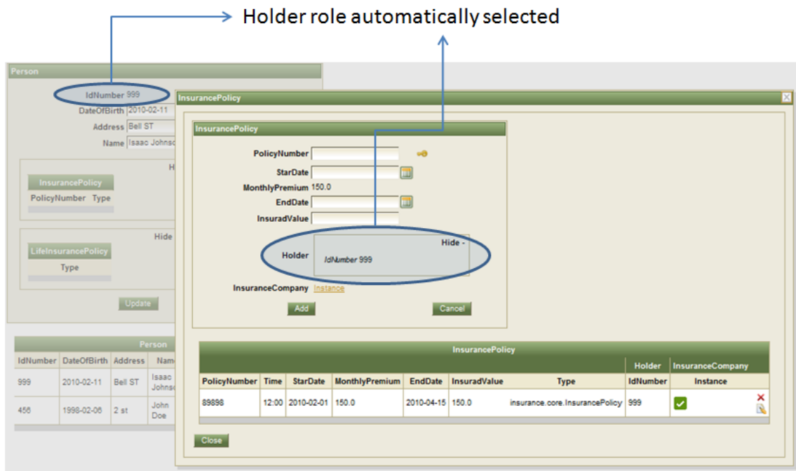
Figure 53. Association panel for the “InsurancePolicy * -- 1 Person holder”
