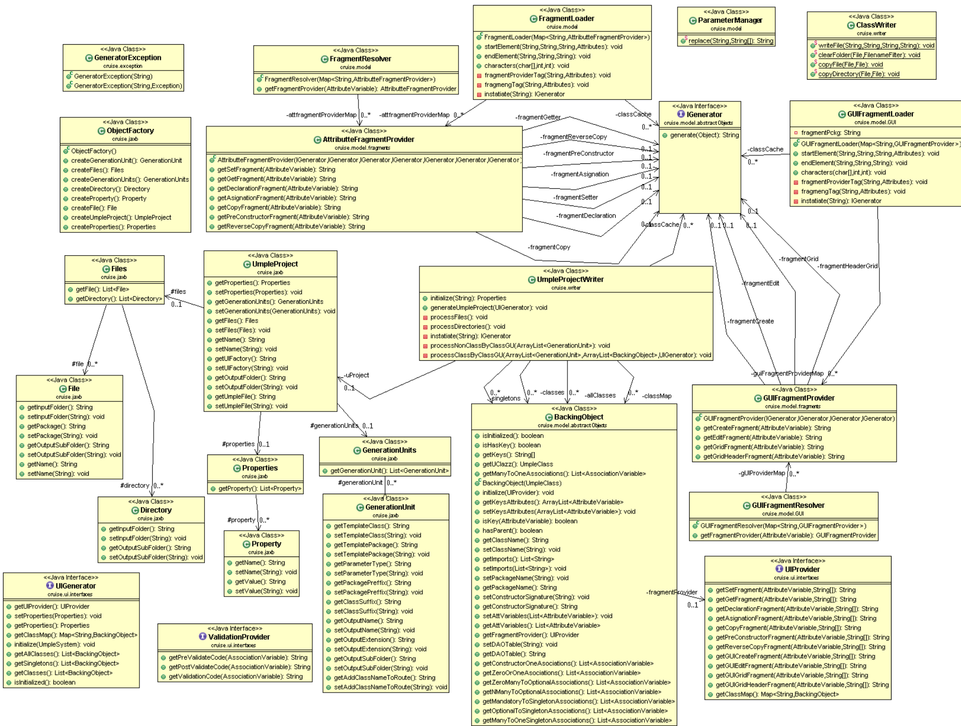
Figure 20. GUIModel class diagram
