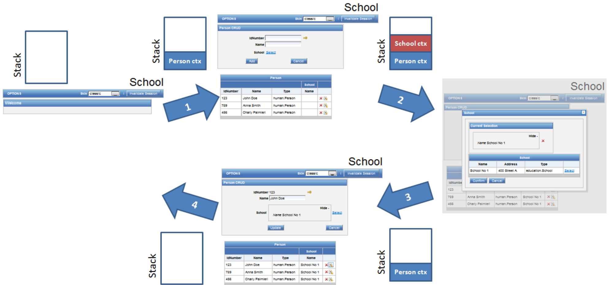
Figure 35. Sample navigation model for the Person -- School model.
