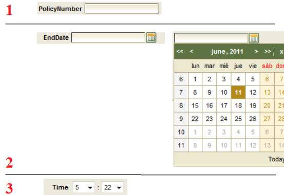
Figure 47. Input components. 1) Textbox for String, Integer and Double attributes, 2) Calendar for Date attributes. 3) Combo boxes for Time attributes
