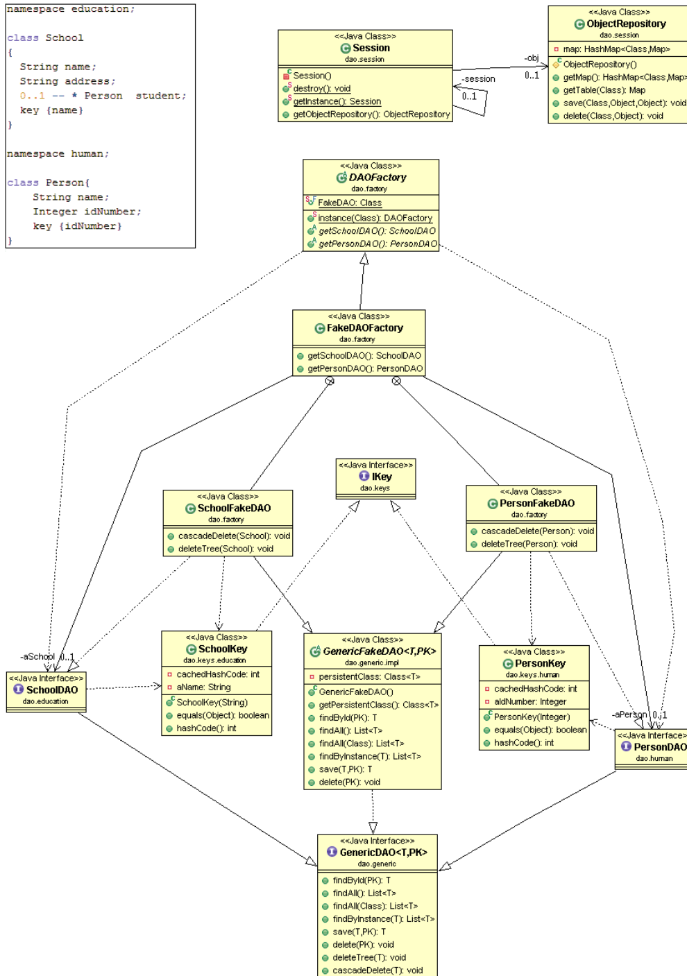
Figure 24. Generated DAO class diagram and Umple model (upper left corner).
