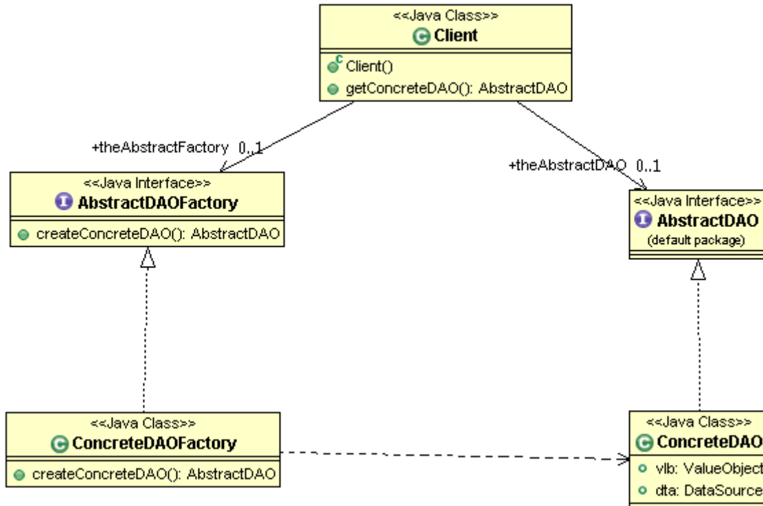
Figure 16. DAO + AbstractFactory, class diagram
