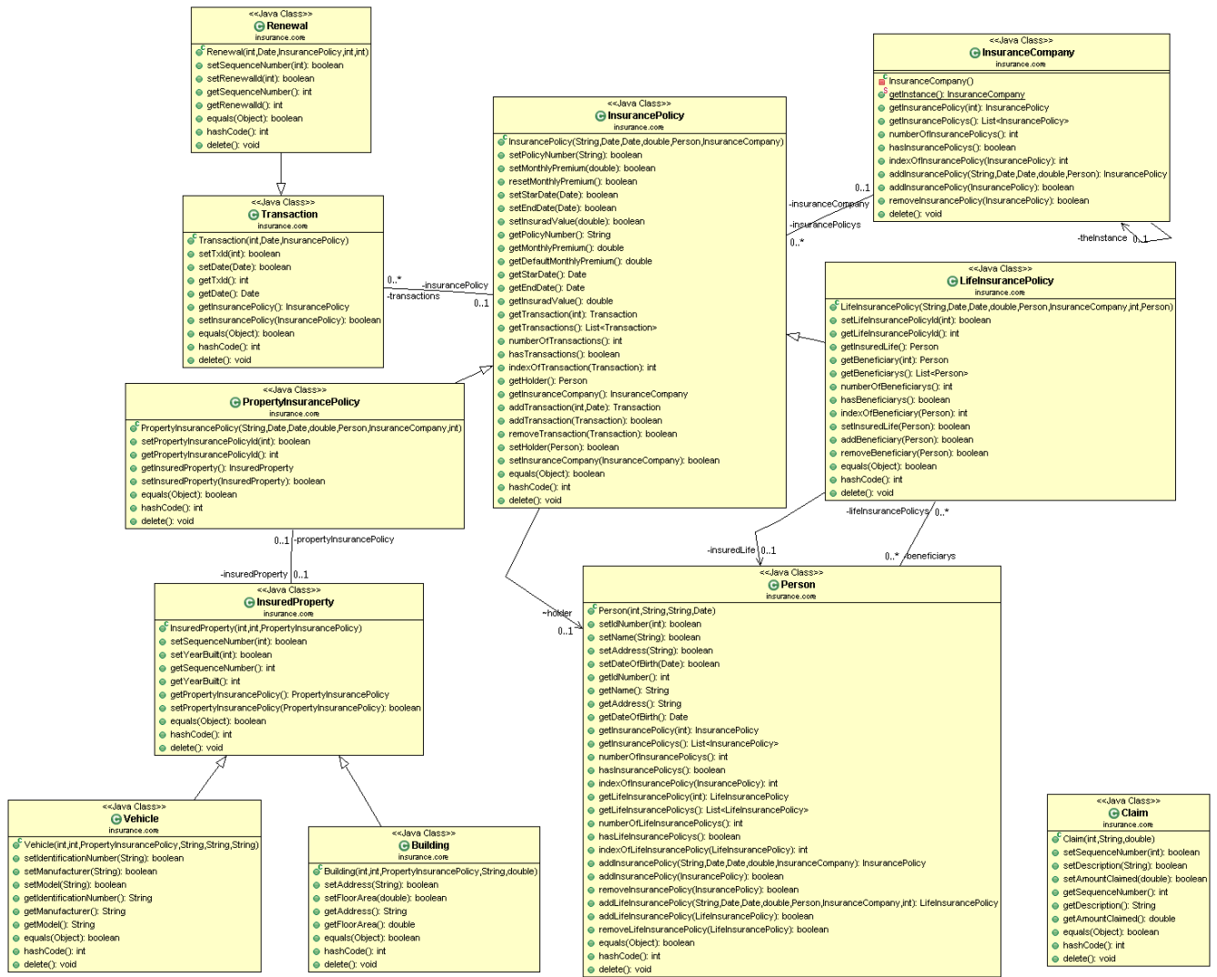
Figure 44. Insurance system class diagram
