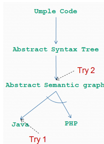
Figure 18. UIGU inputs. Try 1: Uml generated java classes. Try 2: Instances of the Uml metamodel (Abstract semantic graph)
