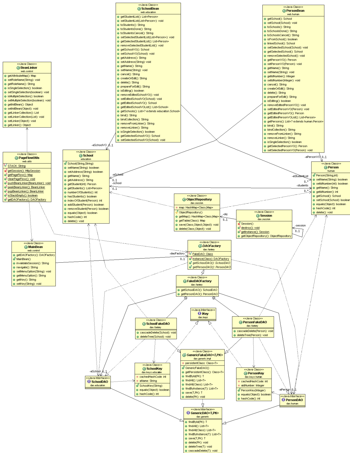
Figure 38. School -- Person model. Generated application's class diagram
