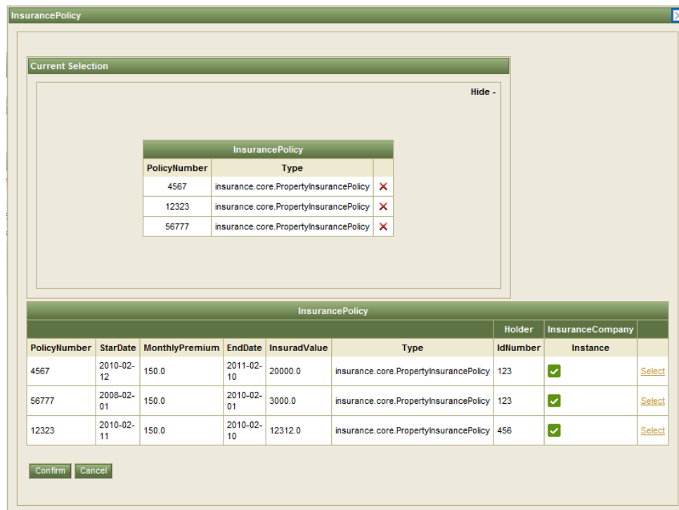
Figure 50. Association Panel for multiple selections
