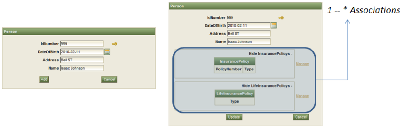
Figure 52. Person CRUD. Create (left),update (right)
